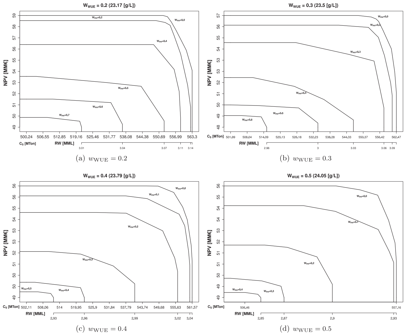
Fig. 5. Pareto fronts of \overline{C}_5 v/s \overline{NPV} for different values of w_{RW} and w_{WUE} \in \{0.2, 0.3, 0.4, 0.5\} .
