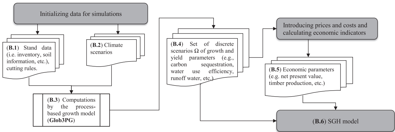
Fig. 1. Block diagram of the decision-making tool.
